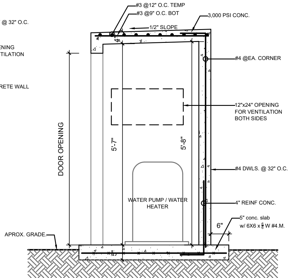
3 PUMP ROOM CROSS SECTION 3/4" = 1'-0"
