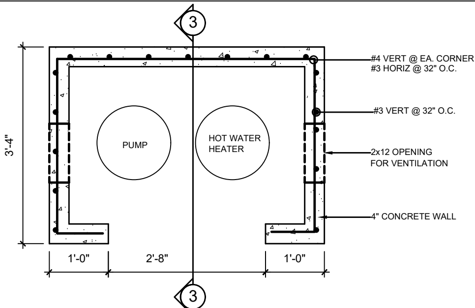
2 PUMP ROOM PLAN 3/4" = 1'-0" 4'-8"
