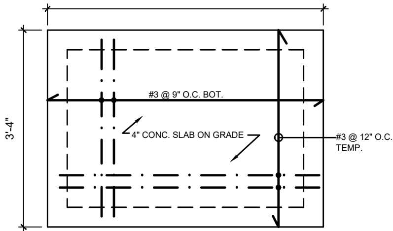
1 STRUCTURAL PLAN 3/4" = 1'-0"
